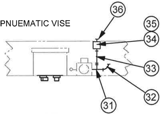
TOP VIEW OF CONTROL PANEL AREA
