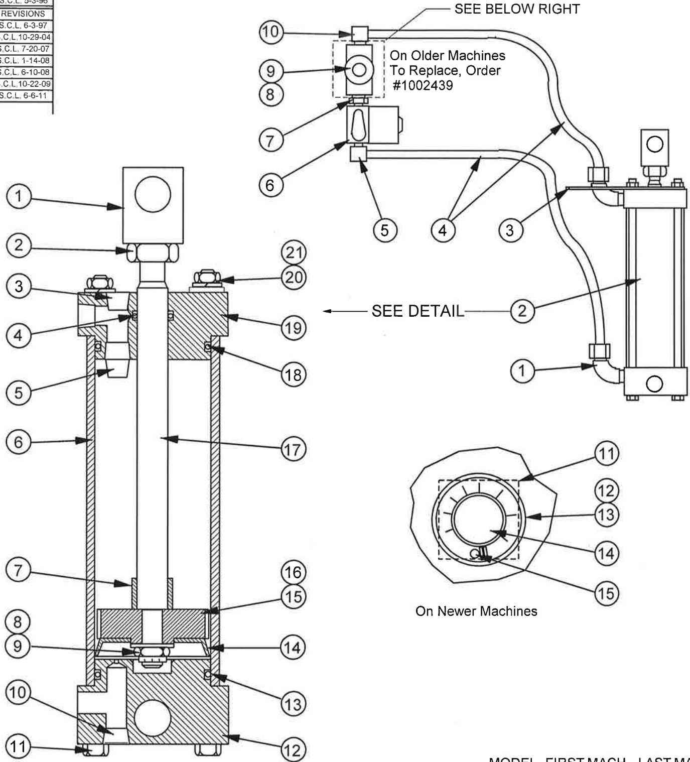
HEAD FEED CYLINDER ASSEMBLY
