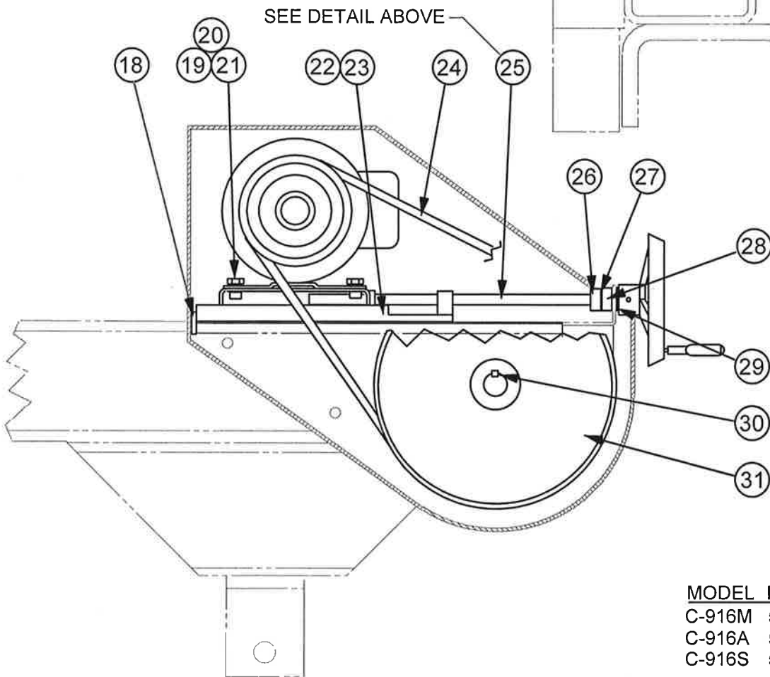
DRIVE ASSEMBLY
